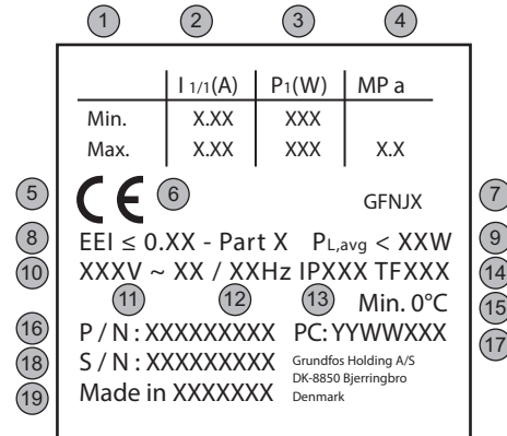
Fig. 8 Terminal box side
