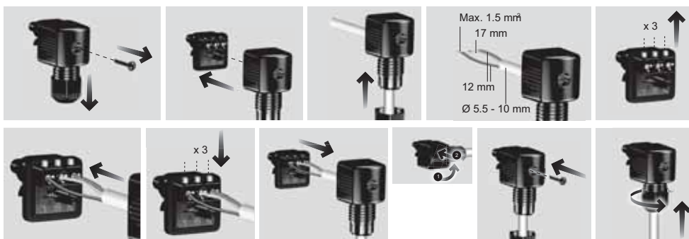
Fig. 67 Superseal installation plug
