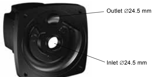
GGBP3 cast-iron, maxi back-panel
