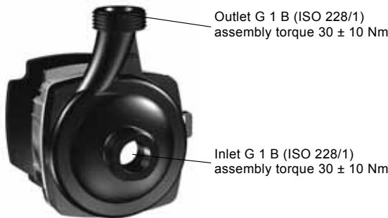
CES3 composite, end-suction
