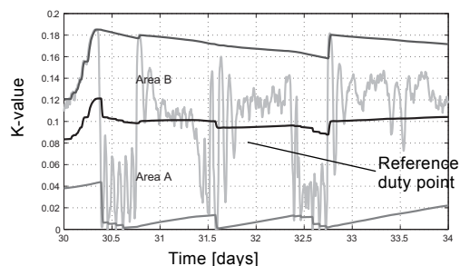
Fig. 32 K_{sys} -values logged for the system analyser
