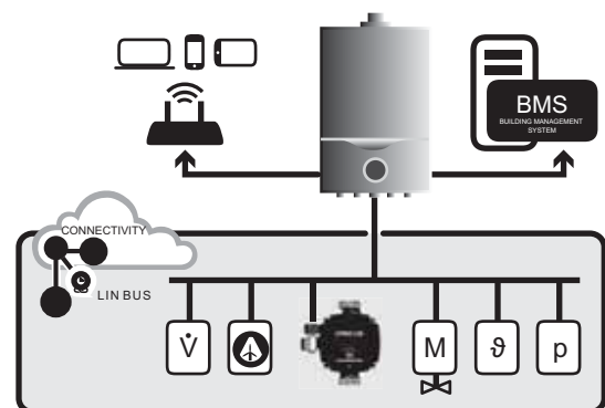
Fig. 20 LIN bus on fieldbus of heating control systems
