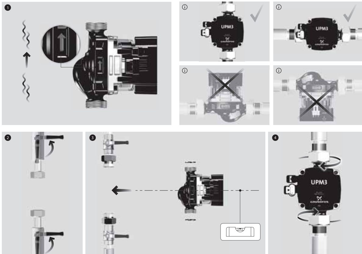
Fig. 52 Mechanical installation
