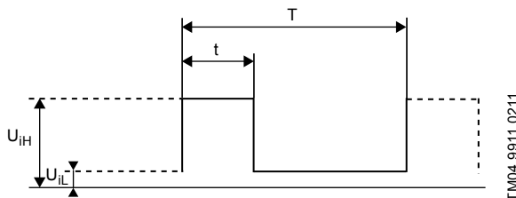
Fig. 12 PWM signal
