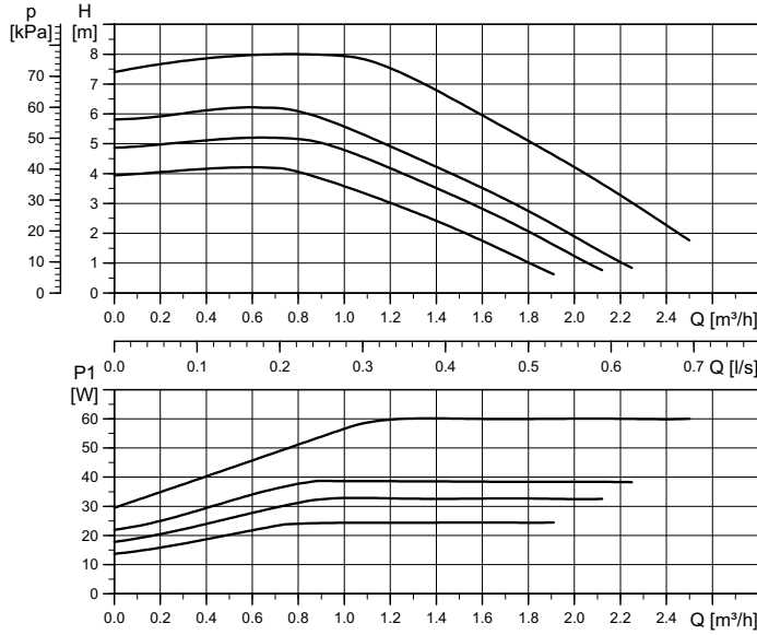
Performance curve
