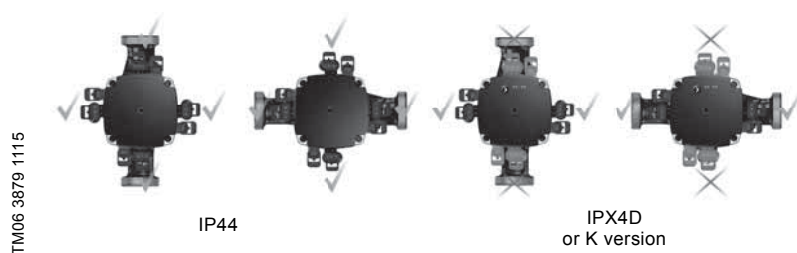
Control box position
