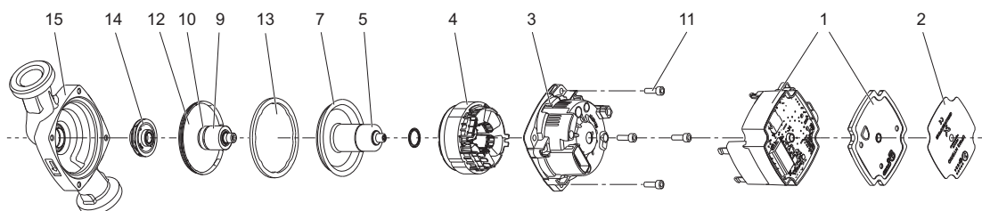
Fig. 35 UPM3 exploded view
