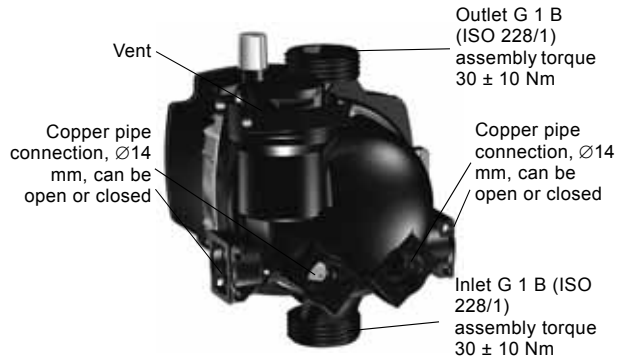
CACAO composite, alternate connection, air outlet
