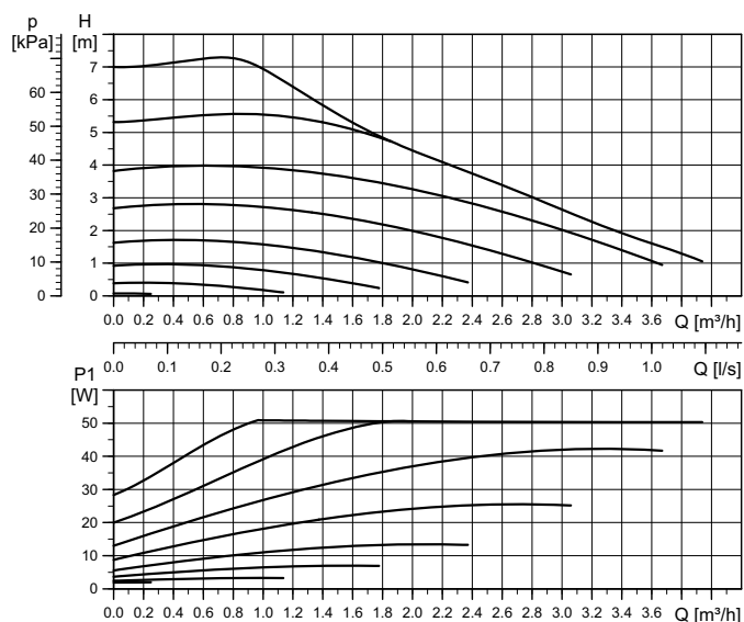
Performance curve
