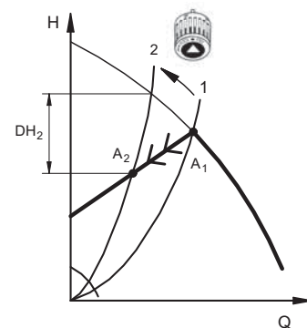
Fig. 28 Pump operated in proportional-pressure control mode
