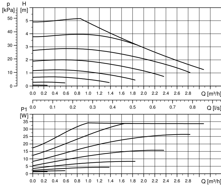
Performance curve
