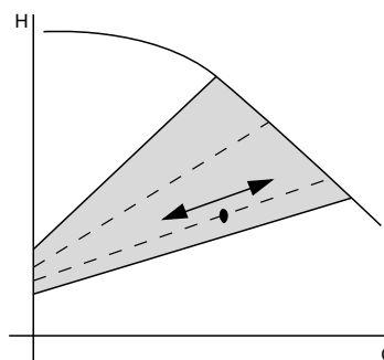
Fig. 34 New lower proportional pressure curve
