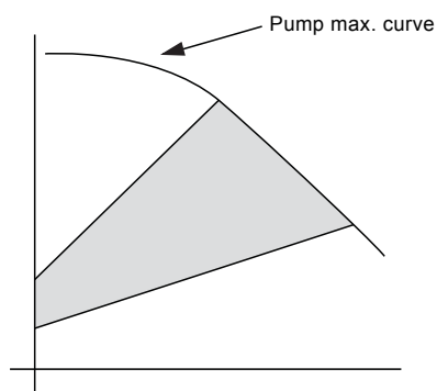
Fig. 30 Proportional pressure AUTO_{ADAPT} operation area
