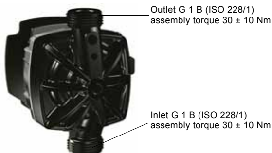
CIL3 composite, inline, 1" x 130 mm
