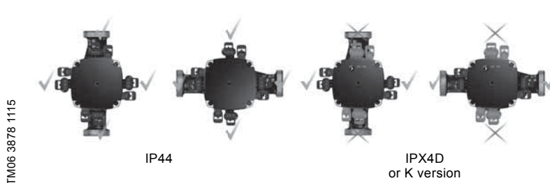
Control box position
