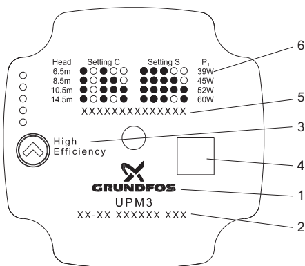
Fig. 6 Nameplate: Grundfos with setting indication
