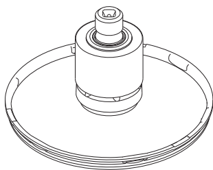
Fig. 46 Moving unit
