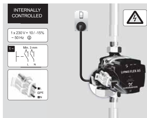
Fig. 64 Control box without signal connection
