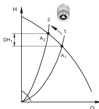
Fig. 27 Uncontrolled pump
