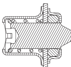
Fig. 41 Sectional drawing of deblocking device
