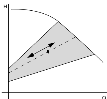
Fig. 31 Proportional pressure control
