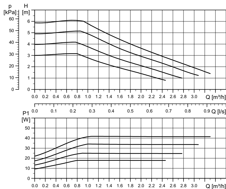
Performance curve
