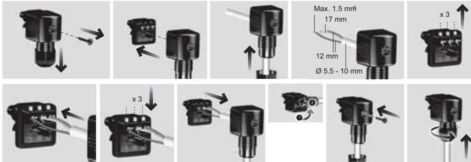
Fig. 67 Superseal installation plug
