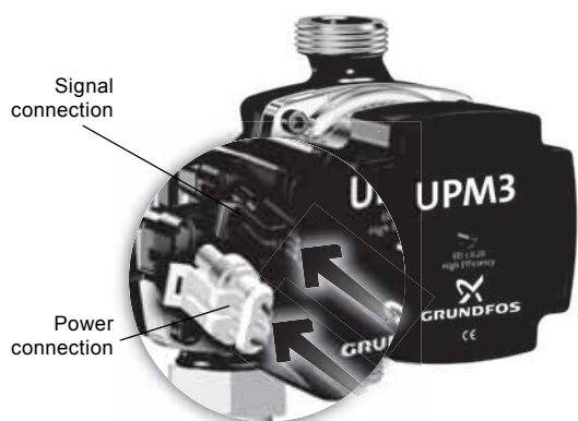
Fig. 61 Signal connection and power connection
