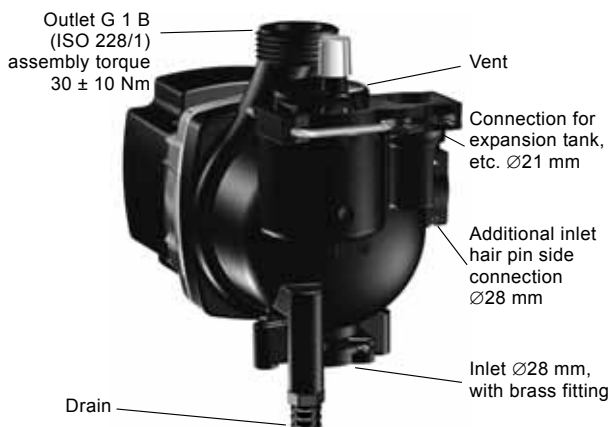
CAOD composite, air outlet, drain
