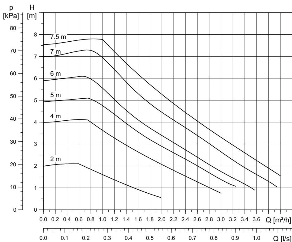
Fig. 9 Performance range UPM3, cast iron pump housing
