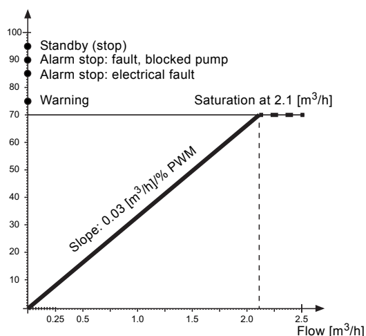
Fig. 18 PWM feedback signal - flow estimation
