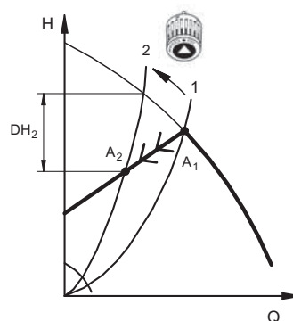
Fig. 28 Pump operated in proportional-pressure control mode
