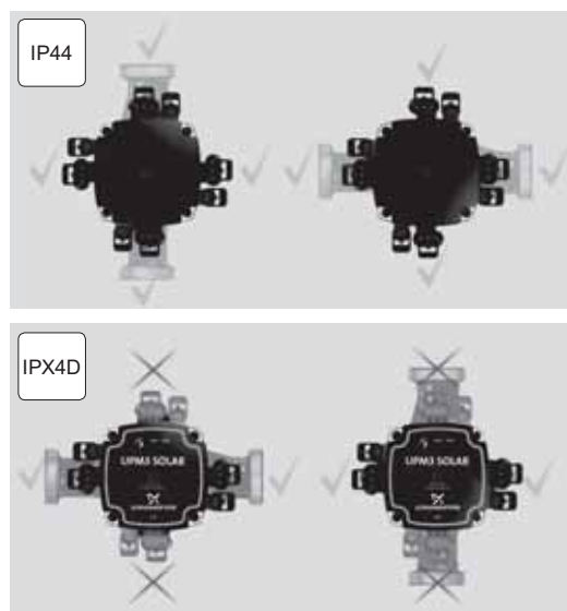
Fig. 53 Control box positions
