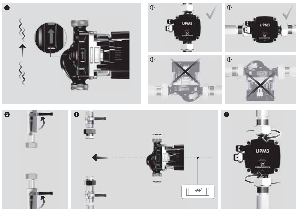
Fig. 52 Mechanical installation
