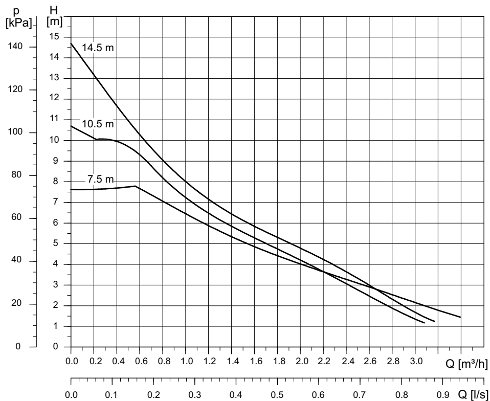
Fig. 10 Performance range UPM3 SOLAR, cast iron pump housing
