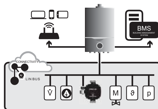
Fig. 20 LIN bus on fieldbus of heating control systems
