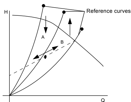
Fig. 33 Duty point on selected proportional pressure curve
