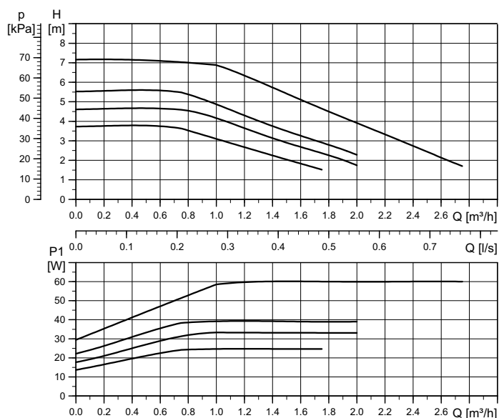
Performance curve
