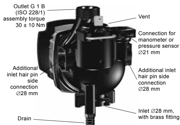
AOKR composite, air outlet, alternate connection, drain
