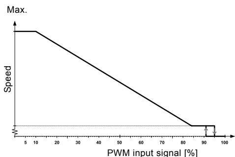
Fig. 14 PWM input profile A (heating)
