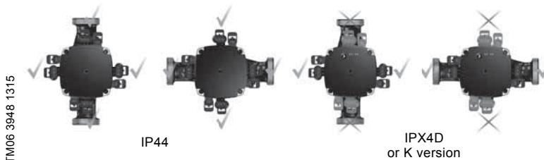
Control box position
