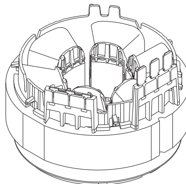
Fig. 38 Stator
