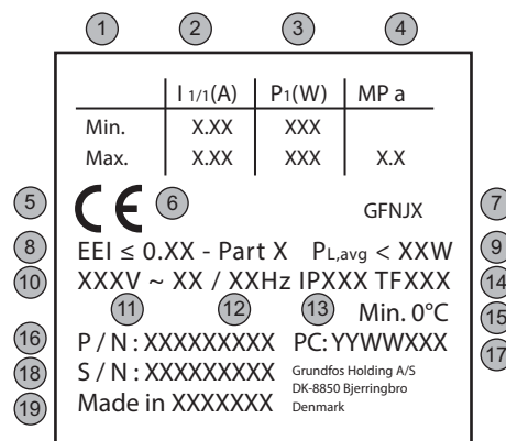
Fig. 8 Terminal box side
