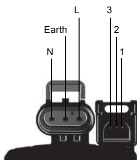
Fig. 62 Connections FCI
