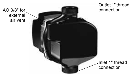
GGAOS3 cast-iron, inline with air outlet
