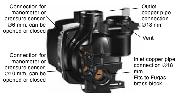
CESAO1 composite, end-suction, air outlet
