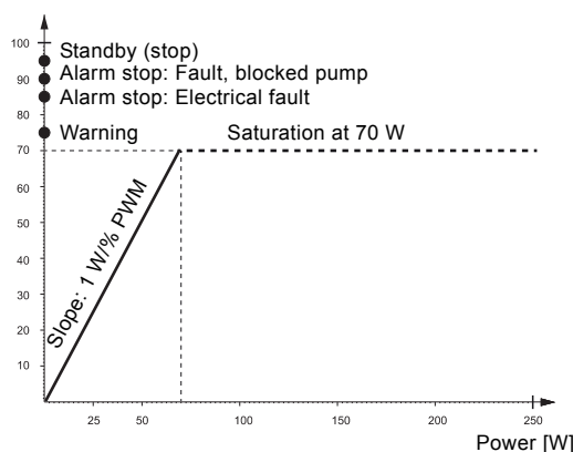
Fig. 16 PWM feedback signal, UPM3 power consumption
