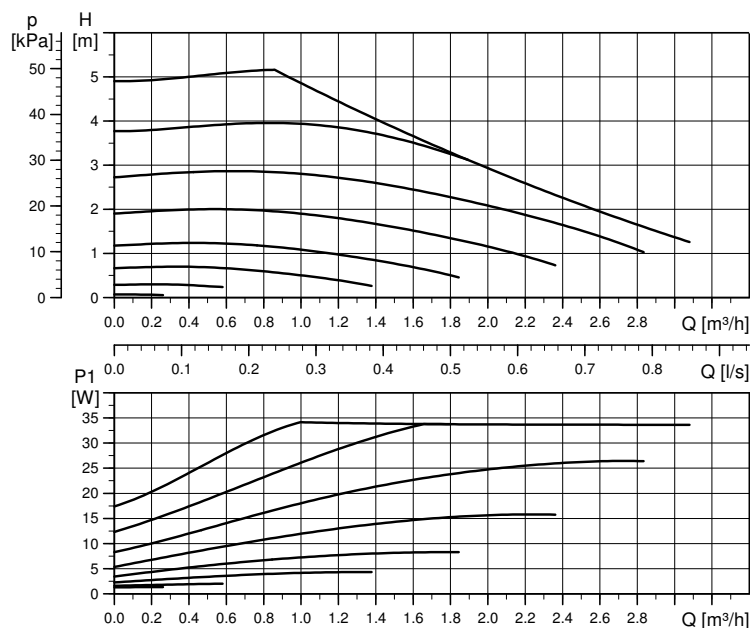
Performance curve
