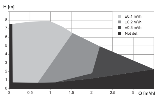
Fig. 19 Accuracy of PWM feedback signal - flow estimation with water at 20 °C
