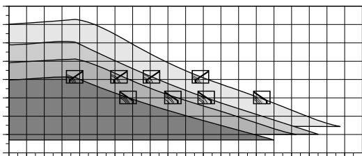
Fig. 26 UPM3 FLEX/HYBRID control modes with pump curves
