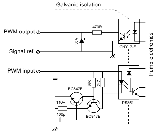
Fig. 13 Schematic drawing, interface
