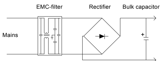
Fig. 57 Rectification of VAC voltage to DC voltage
