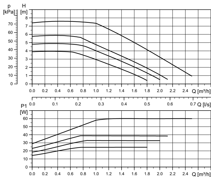
Performance curve
