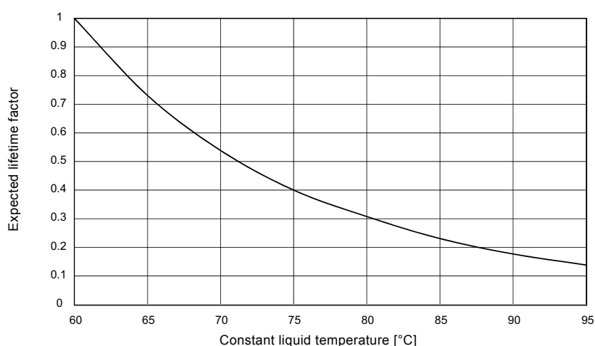
Fig. 51 Diagram temperature/expected lifetime for PA 6.6 30 % GF
