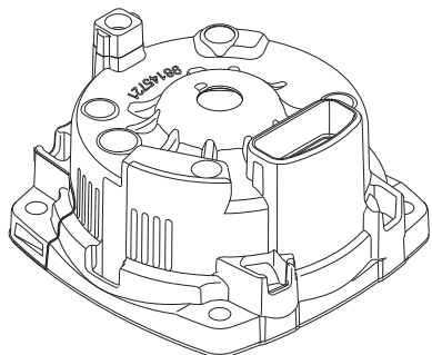
Fig. 37 Stator housing
