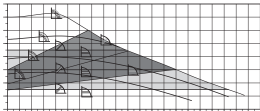
Fig. 25 UPM3 AUTO/HYBRID control modes with pump curves
