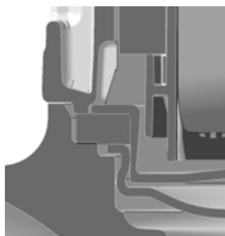
Fig. 48 Sectional drawing showing sealing principle of gasket
