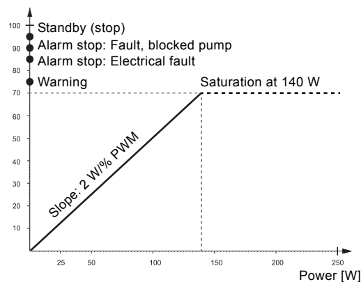
Fig. 17 PWM feedback signal, UPM3L power consumption
