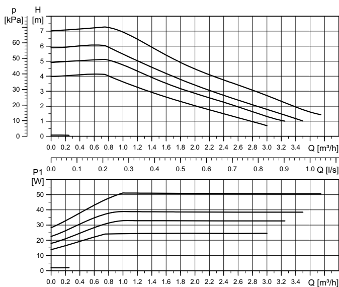
Performance curve
