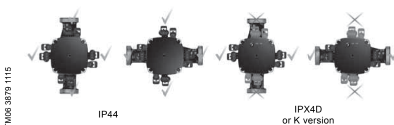
Control box position
