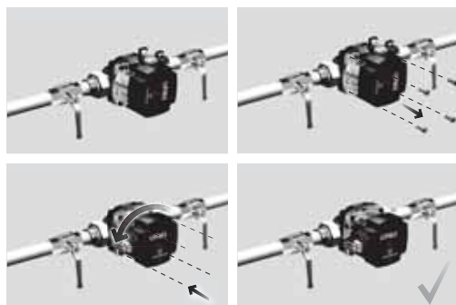
Fig. 54 Changing the control box position
