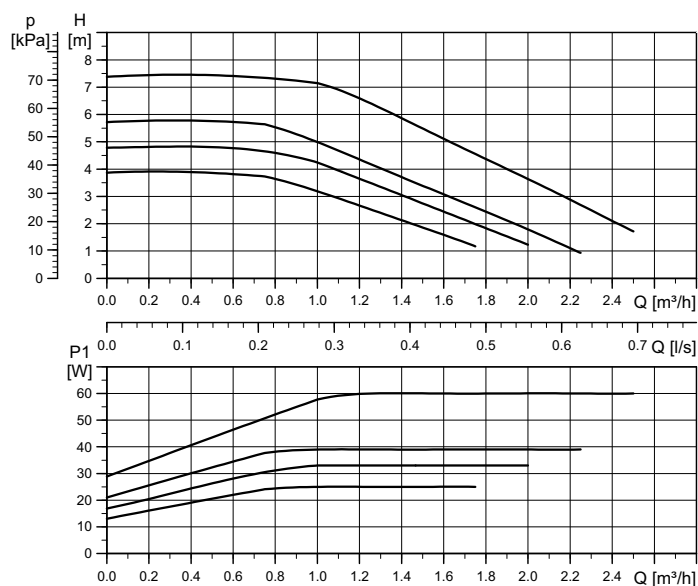
Performance curve
