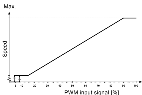
Fig. 15 PWM input profile C (solar)
