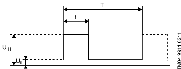
Fig. 12 PWM signal
